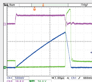
Measurement Waveform
