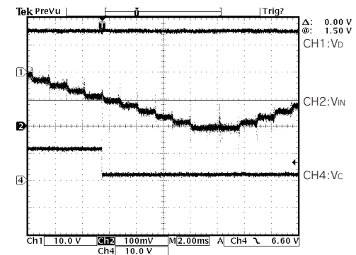
[Expanded waveform of V CIN(ON) ] [V CIN(ON) 拡大波形]
