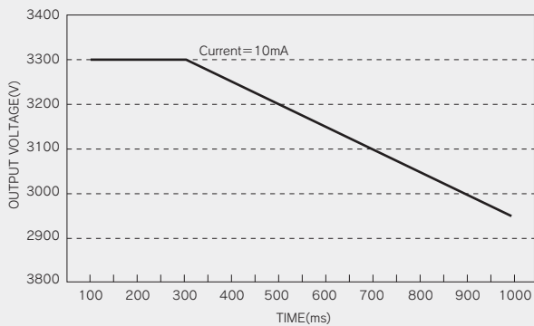
Power area of high voltage supply (高圧電源パワーエリア)
