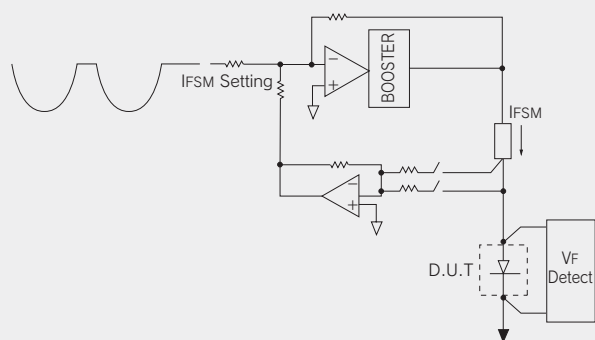
Fundamental Test Circuit
