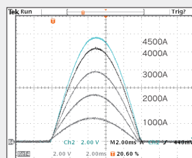
Measurement Waveform
