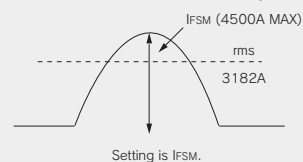
Measurement Waveform
